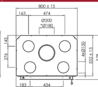
Swing Front 67x57 (P. 52) Varia 1V-57-4S
