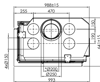
Premium Corner 80x40x50 (P. 36) Premium V-2L/2R-80h
